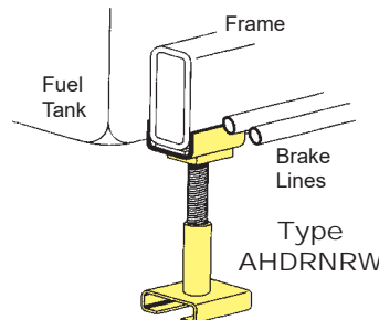
Opening Dimensions: 4-1/4" x 1-1/8"
