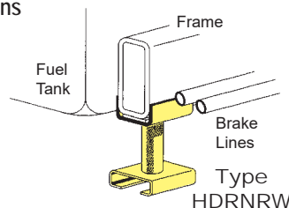
Opening Dimensions: 5-3/16" x 25/32"
