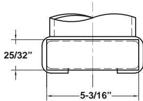
Adapter Base Inside Dimensions Shape may vary depending on height extension.
