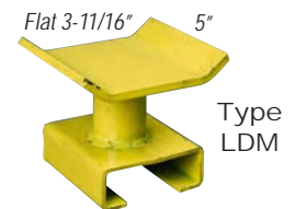
Opening Dimensions: 5-3/16" x 25/32"
