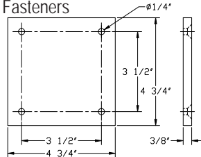
4-3/4" x 4-3/4" Square
