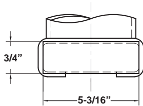
Adapter Base Inside Dimensions Shape may vary depending on height extension.
