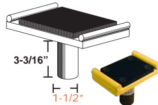
Replacement Rubber Pad: BH-7536-92P Pad Dimensions: 4-1/8" x 3-1/4"
