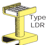
Opening Dimensions: 4-1/4" x 1-1/8"
