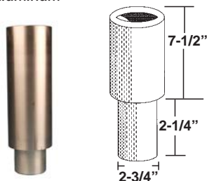
BH-7536-55 (Ref FJ7822-6) 7-1/2" Nesting Height Extension Aluminum
