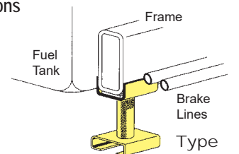
Opening Dimensions: 4-1/4" x 1-1/8"
