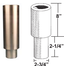
BH-9791-43 (Ref FD2338) 8" Nesting Style Height Extension - Aluminum
