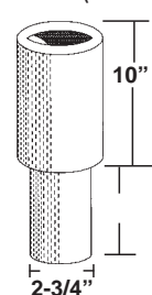
10" Nesting Style Height Extension BH-7548-029 (Ref FJ71014)
