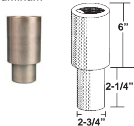
BH-7536-53B 6" Nesting Height Extension Aluminum
