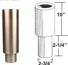
BH-7536-54 (Ref FJ7822-5) 10" Nesting Height Extension Aluminum
