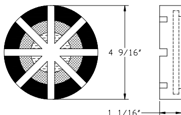
4-9/16" OD 4" ID Bottom Side with lip
