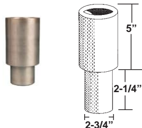
BH-7536-53 (Ref FJ7822-4) 5" Nesting Height Extension Aluminum
