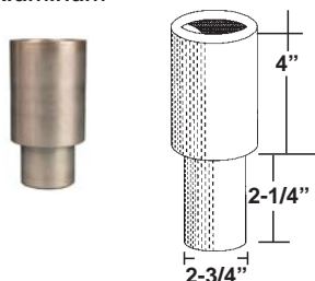
BH-7536-53A 4" Nesting Height Extension Aluminum
