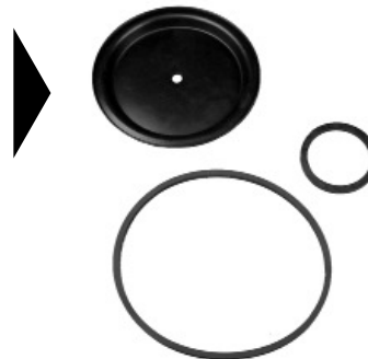
BP-4128 Diaphragm for Tokheim 786, 787, 788 (Ref # 1-223889)
