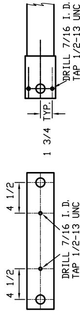
Carriage Crossarm - Bottom
